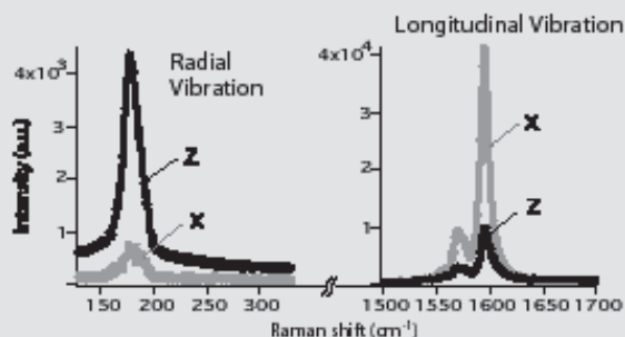
Tip-enhanced Raman spectra of carbon nanotubes
