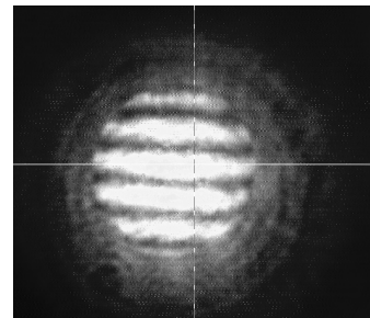
FC100 interferogram of whole aperture at 1550nm.
