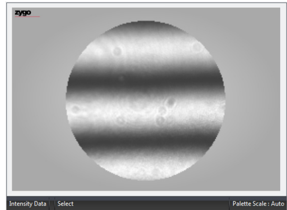
FC100 interferogram of whole aperture at 1550nm.
